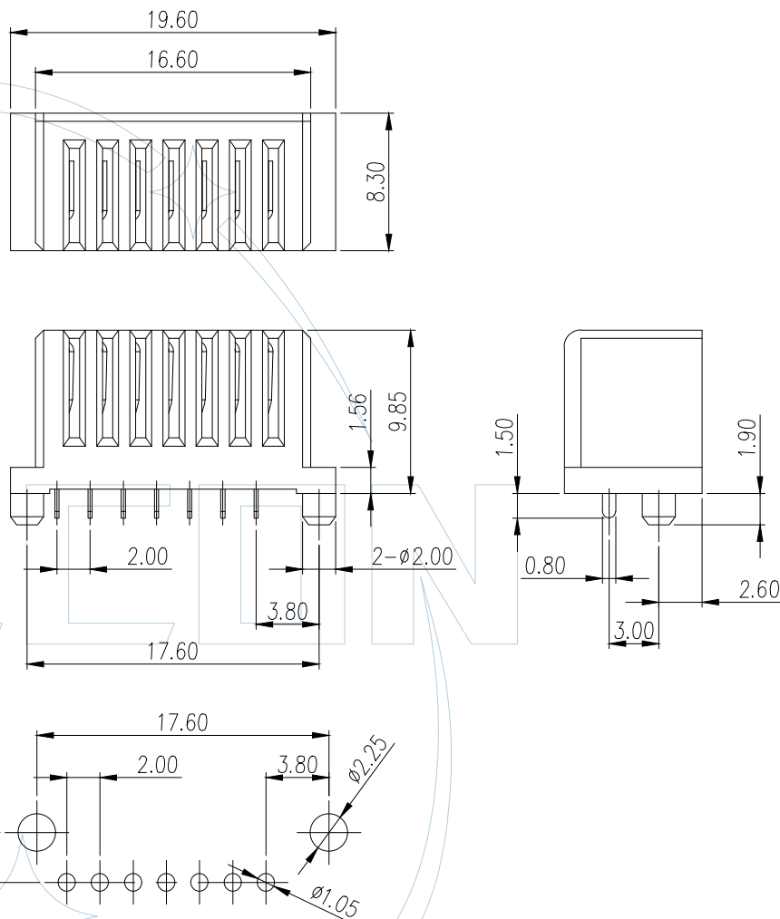
Recommended P.C.Board Layout Layout Tolerance: ± 0.05 mm
