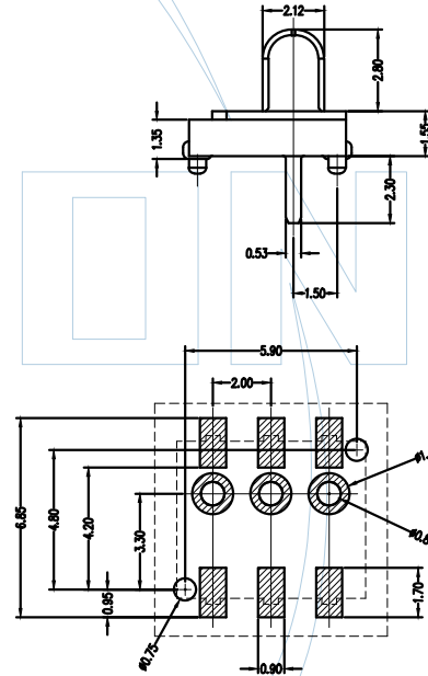
Recommended P.C.Board Layout Layout Tolerance: ±0.05mm
